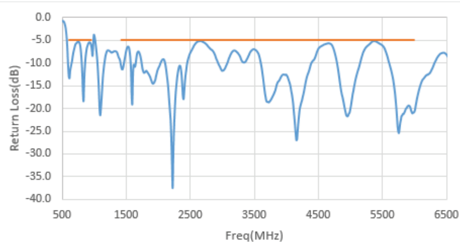
Return Loss
