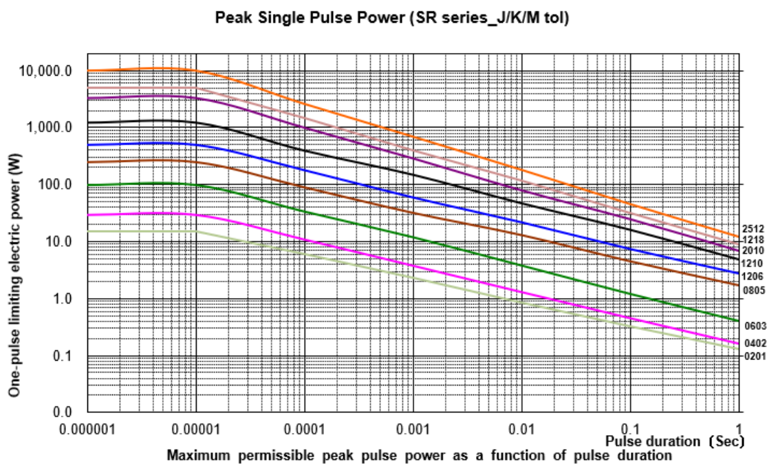
Fig. 7-2 Pulse-Load behavior
