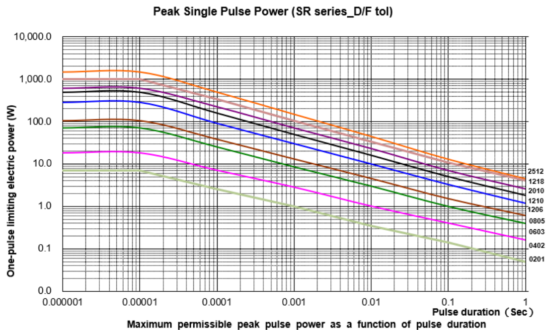
Fig. 7-1 Pulse-Load behavior
