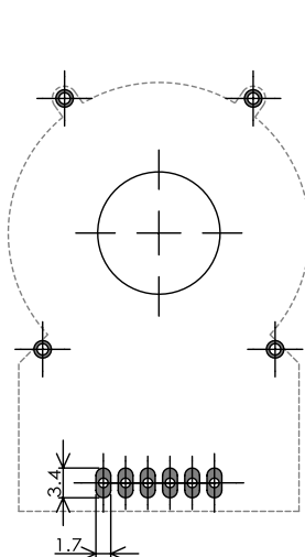
Solder Side
