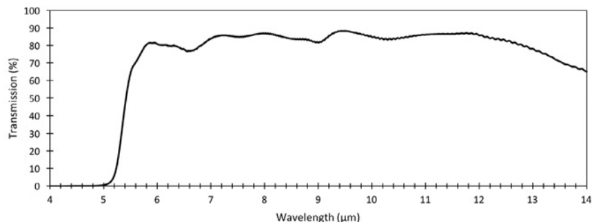
Typical 5.0 \mu\text{m} LP Filter Transmission
