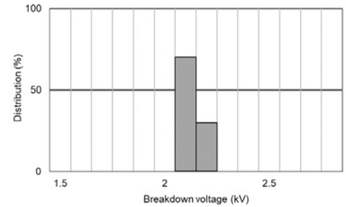
(b) Between adjacent contacts
