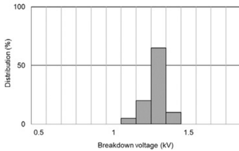
(a) Between open contacts
