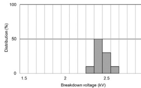
(c) Between coil and contacts
