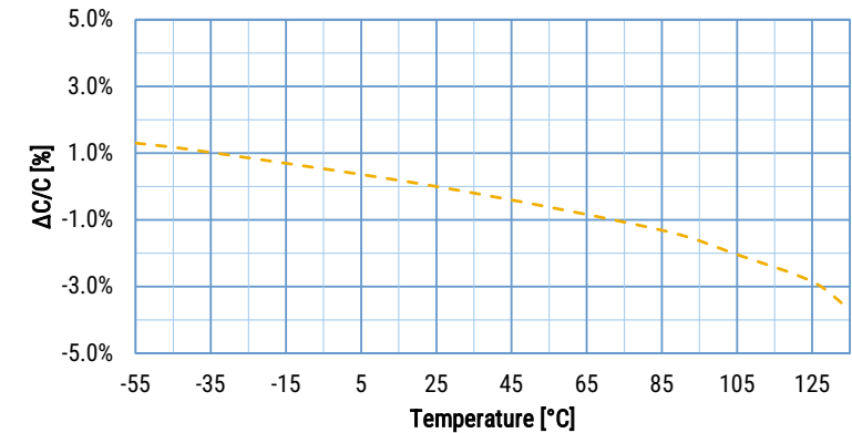
Typical Capacitance vs. Temperature at 1kHz
