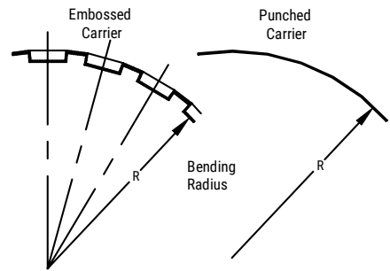
Figure 4 – Bending Radius
