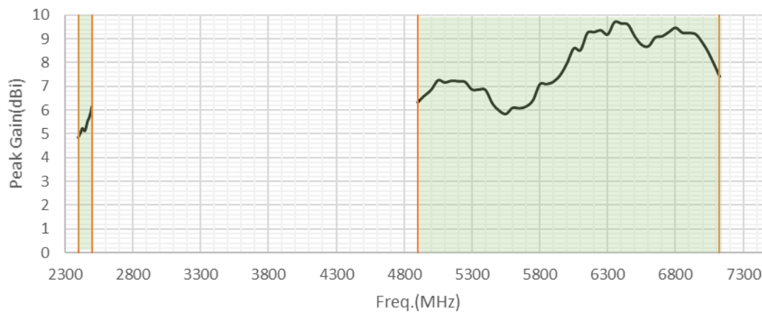
Peak Gain vs Frequency
