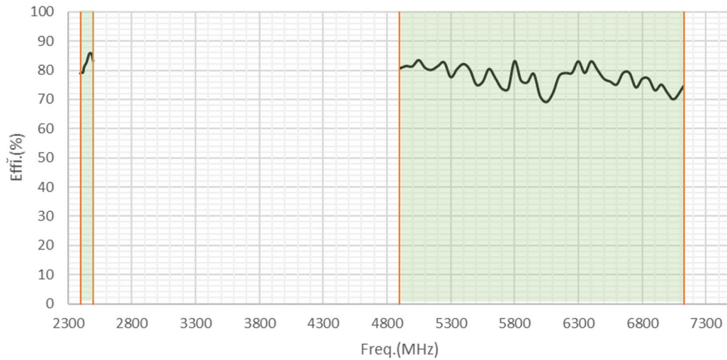
Efficiency vs Frequency
