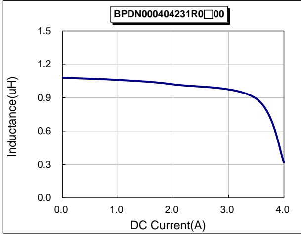
INDUCTANCE vs. DC CURRENT @100kHz/0.25V
