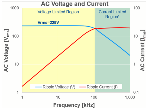
Figure 2 – AC Voltage VS AC Current limited regions
