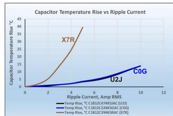
Figure 1 – Temperature rise comparison by dielectrics.
