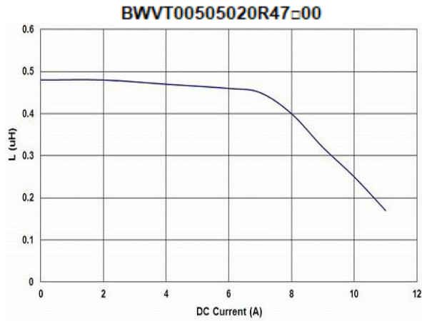
13 Graph: BWVT00505020 Series Graph
