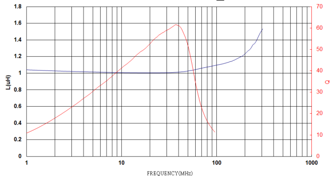
AWLS003025221R5□00
