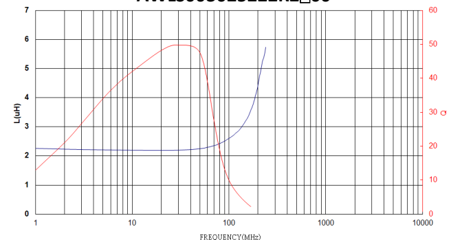
AWLS003025222R2□00
