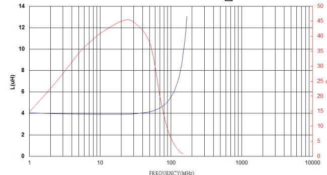
AWLS003025223R9□00
