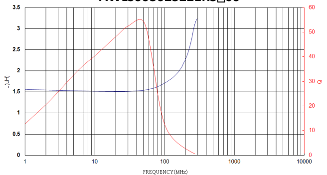
AWLS003025222R2□00
