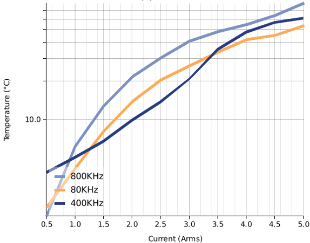
Ripple Current
